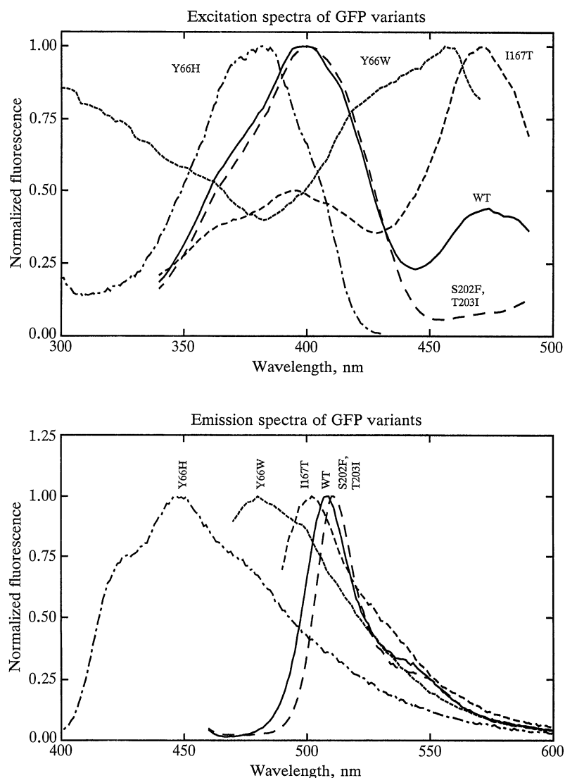
FIG. 3. Excitation and emission spectra of Wild-type and mutant GFPs. —, Wild-type; —, mutations S202F, T203I; ---, mutation I167T; ·····, mutation Y66W; —·—, mutation Y66H. Samples were soluble fractions from E. coli expressing the proteins at high level, except for mutant Y66W, which was obtained in very low yield and measured on intact cells. Autofluorescence was negligible for all spectra except those of mutant Y66W, whose excitation spectrum below 380 nm may be contaminated by autofluorescence. All amplitudes have been arbitrarily normalized to a maximum value of 1.0. To compare brightnesses at equal protein concentrations, see Table 1.
