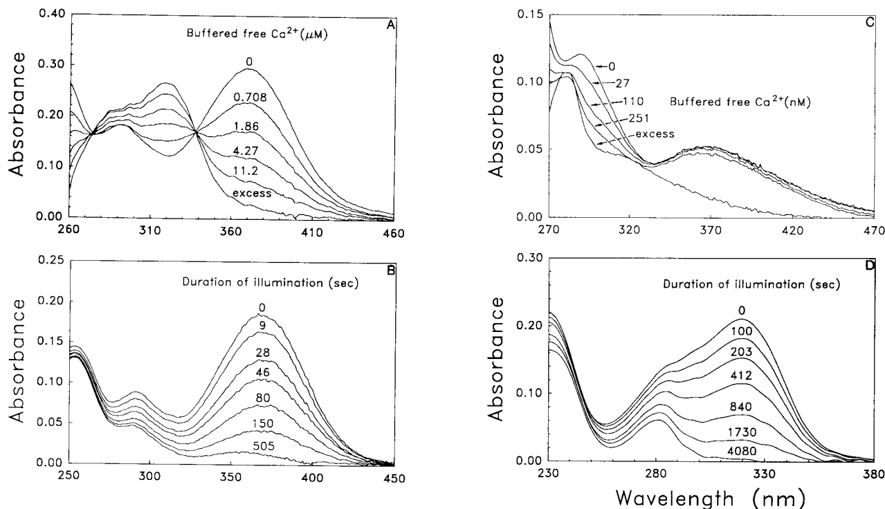
Figure 1. (A) Absorbance spectra of unphotolyzed diazo-2 as a function of free [\text{Ca}^{2+}] . The titration was done at 22 °C with 10 mL of 100 mM KCl, 10 mM K-MOPS, 10 mM \text{K}_2\text{H-HEEDTA} , and 14 \mu\text{M} diazo-2 as starting materials, adjusting the pH to 7.24, recording the spectrum, and then discarding 1.0 mL of this solution and replacing with 1.0 mL of 100 mM KCl, 10 mM K-MOPS, 10 mM \text{KCa-HEEDTA} , 14 \mu\text{M} diazo-2, readjusting the pH to 7.24, and recording the spectra, which was then in 9 mM \text{K}_2\text{H-HEEDTA} . Subsequent iterations to reach n mM \text{KCa-HEEDTA} , (10 - n) mM \text{HEEDTA} , n = 2-10 , were done by discarding 10.0/(11 - n ) mL and replacing with equal volumes of the 10 mM \text{KCa-HEEDTA} , 14 \mu\text{M} diazo-2 stock. After n = 10 had been reached to give a free \text{Ca}^{2+} between 10^{-5} and 10^{-4} M, addition of 1 mM \text{CaCl}_2 had no further effect on the spectrum. For clarity, only six spectra are included in the figure, n = 0, 2, 4, 6, 8 , and 10. Each spectrum is labeled with the calculated free [\text{Ca}^{2+}] imposed by the \text{HEEDTA} buffer, assuming a log effective stability constant 39 of 5.55 at pH 7.24. (B) Absorbance spectra of diazo-2 undergoing photolysis in the absence of \text{Ca}^{2+} . Diazo-2 was dissolved at 8 \mu\text{M} in 100 mM KCl, 10 mM Tris, 5 mM MOPS, 4 mM \text{K}_2\text{H}_2\text{EGTA} and pH titrated to 7.2 with HCl. Spectra were obtained after 0, 2, 5, 9, 16, 28, 46, 80, 150, 285, 505, and 903 s of 365-nm illumination at 7.82 \times 10^{-9} einstein \text{cm}^{-2} \text{s}^{-1} from the Spectroline lamp. For clarity only the 0-, 9-, 28-, 46-, 80-, 150-, and 505-s spectra have been reproduced here. The 505- and 903-s spectra were identical, confirming completion of photolysis after those times. Solutions were at 22 \pm 2 °C. (C) Absorbance spectra of phenylacetate (photolyzed diazo-2) as a function of free [\text{Ca}^{2+}] . The phenylacetate was produced by irradiating a 30 \mu\text{M} solution of diazo-2 in 100 mM KCl, 10 mM Tris-HCl, 10 mM \text{K}_2\text{H-HEEDTA} , pH 8.40, with the Spectroline lamp at 365 nm to completion. The titration was then performed as in A but the pH was maintained at 8.40, at which the calculated log effective stability constant 39 for \text{HEEDTA} was 6.60. (D) Absorbance spectra during photolysis of the \text{Ca}^{2+} complex of diazo-2. The method was as described in B except that the \text{EGTA} was replaced by 2 mM \text{CaCl}_2 , and spectra were measured after 0-, 50-, 100-, 203-, 412-, 840-, 1730-, 4080-s illumination. The last two spectra were identical, confirming completion. For clarity, the 50- and 8000-s spectra have been omitted.
