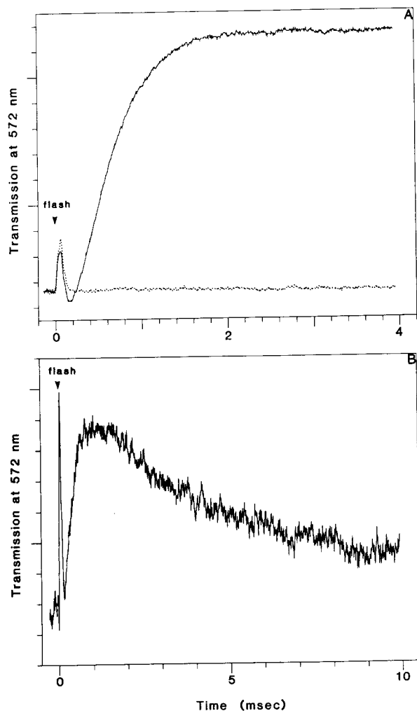
Figure 2. (A) Kinetics of generating high-affinity chelator as signaled by acid release following flash photolysis of diazo-2. Diazo-2 was dissolved at 70 \mu\text{M} concentration in 100 mM KCl, 40 \mu\text{M} BAPTA, and enough cresol red to yield \text{OD}_{572} = 0.1 after the solution has been adjusted to pH 8. Transmitted light intensity at 572 nm was monitored by use of an Hg-Xe arc lamp, a monochromator, a photomultiplier, and a Biomation transient recorder. Each small division of the ordinate corresponds to 0.002 absorbance unit. The small upward spike at time zero is an optical artifact from the xenon flash lamp. The solid trace is from the sample containing diazo-2. For comparison, the dotted trace is from a photochemically inert sample containing cresol red in 100 mM KCl at pH \sim 8 . This control record shows that the flash artifact is clearly separable from the gradual decrease in absorbance of the cresol red as acid is released during the dark reaction following flash photolysis of diazo-2. (B) Kinetics of \text{Ca}^{2+} uptake by photolyzed diazo-2. The sample contained 70 \mu\text{M} diazo-2, 2 mM HEEDTA, 1 mM \text{CaCl}_2 , 100 mM KCl, and cresol red to give \text{OD}_{572} = 0.1 after the solution was adjusted to pH 8 under helium purge. Monitoring of the light transmission at 572 nm was performed as for A. Each small division of the ordinate corresponds to 3.4 \times 10^{-4} absorbance unit. The spike at time zero is an optical artifact generated by the xenon flash lamp. As the acid form of the high-affinity chelator was generated following flash photolysis, the solution transiently acidified, as revealed by the decrease in cresol red absorbance (rise in transmitted light intensity). As the photolyzed diazo-2 took \text{Ca}^{2+} away from HEEDTA, the freed HEEDTA bound protons and thus alkalinized the solution, a process reflected by the increase in cresol red absorbance (decline in light transmission at 572 nm).
