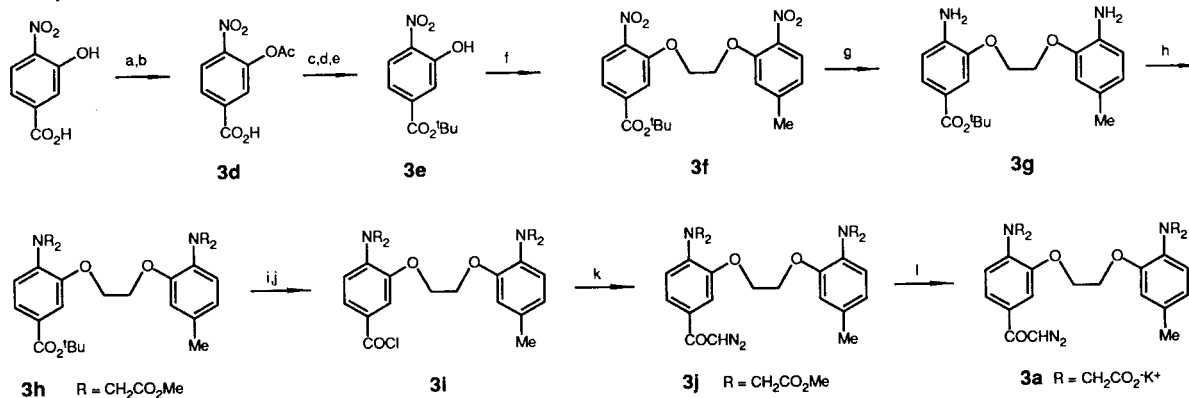
Scheme IV. Synthesis of Diazo-2 a
