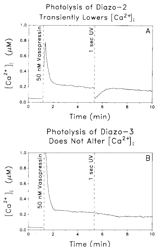
Figure 3. (A) Rapid \text{Ca}^{2+} sequestration by flash-photolyzed diazo-2 in a Fisher rat embryo fibroblast cell. Prior to the start of data acquisition, the REF52 fibroblast cell was loaded with fluo-3 and diazo-2 by incubation for 30 min at 25 °C in DME medium containing 1 \mu\text{M} diazo-2 AM and 10 \mu\text{M} fluo-3/AM. Acquisition of fluo-3 fluorescence intensity images was begun at time 0. The fluorescence intensity data were converted to intracellular \text{Ca}^{2+} concentrations by a calibration procedure previously described. 9b The event markers correspond to (1) stimulating the cell with 50 nM [\text{Arg}^8]\text{vasopressin} and (2) flashing the cell for 1 s with UV light. (B) A control experiment to show that the [\text{Ca}^{2+}] drop in (A) required the entire \text{Ca}^{2+} -binding site of diazo-2 and was not an artifact arising from the chemistry of diazoacetyl group photolysis. The experimental conditions were the same as in (A) except that the cell was loaded with fluo-3 and diazo-3 (instead of diazo-2) by incubation for 90 min at 25 °C in DME medium containing 10 \mu\text{M} fluo-3/AM and 1 \mu\text{M} diazo-3/AM. The event markers correspond to (1) stimulating the cell with 50 nM [\text{Arg}^8]\text{vasopressin} and (2) flashing the cell for 1 s with UV light.
